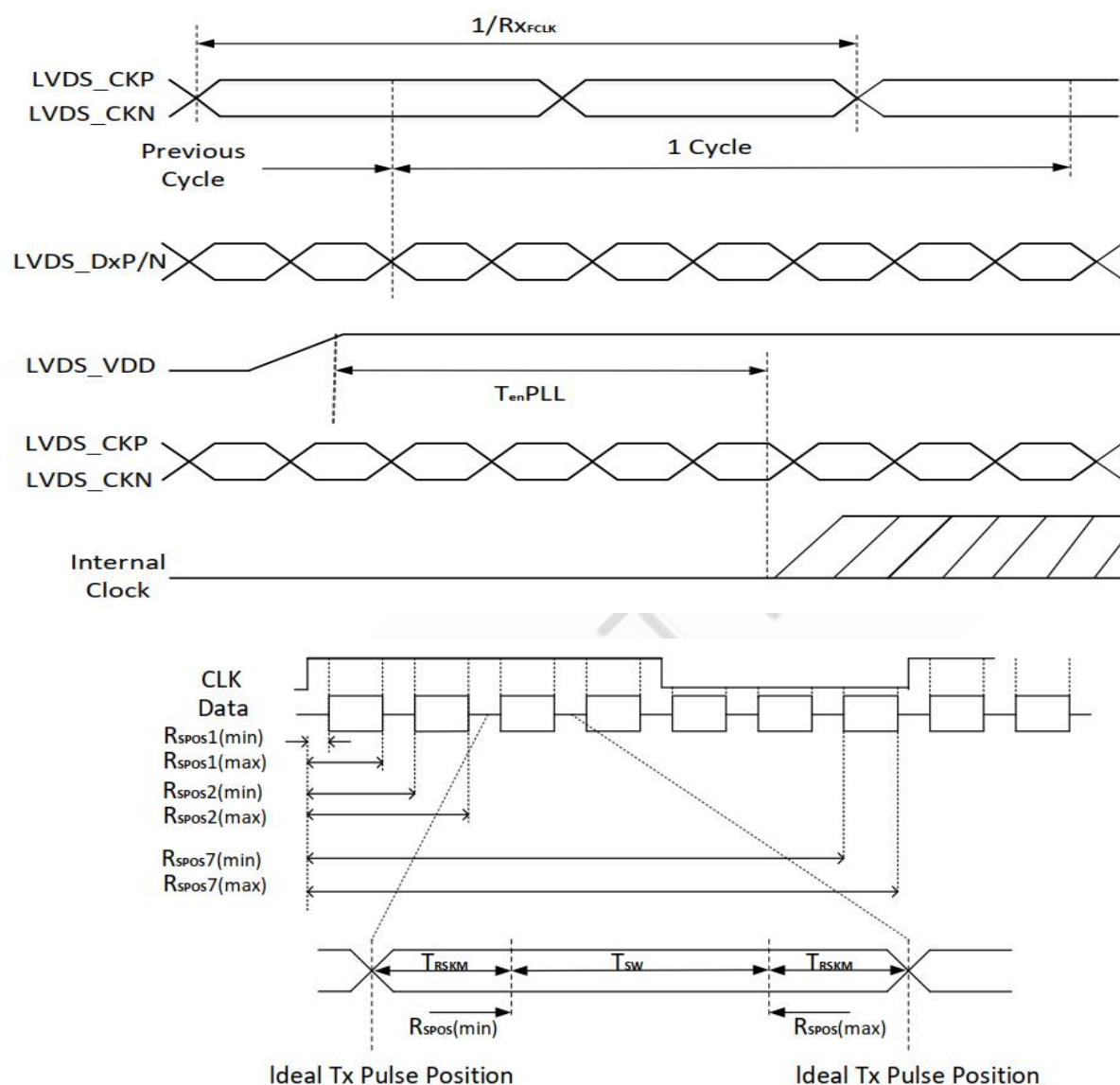
Figure 10.4: LVDS AC characteristics
