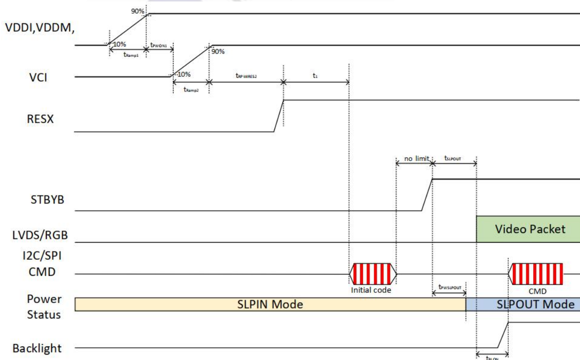
LVDS 接口上电 LVDS Interface power on
