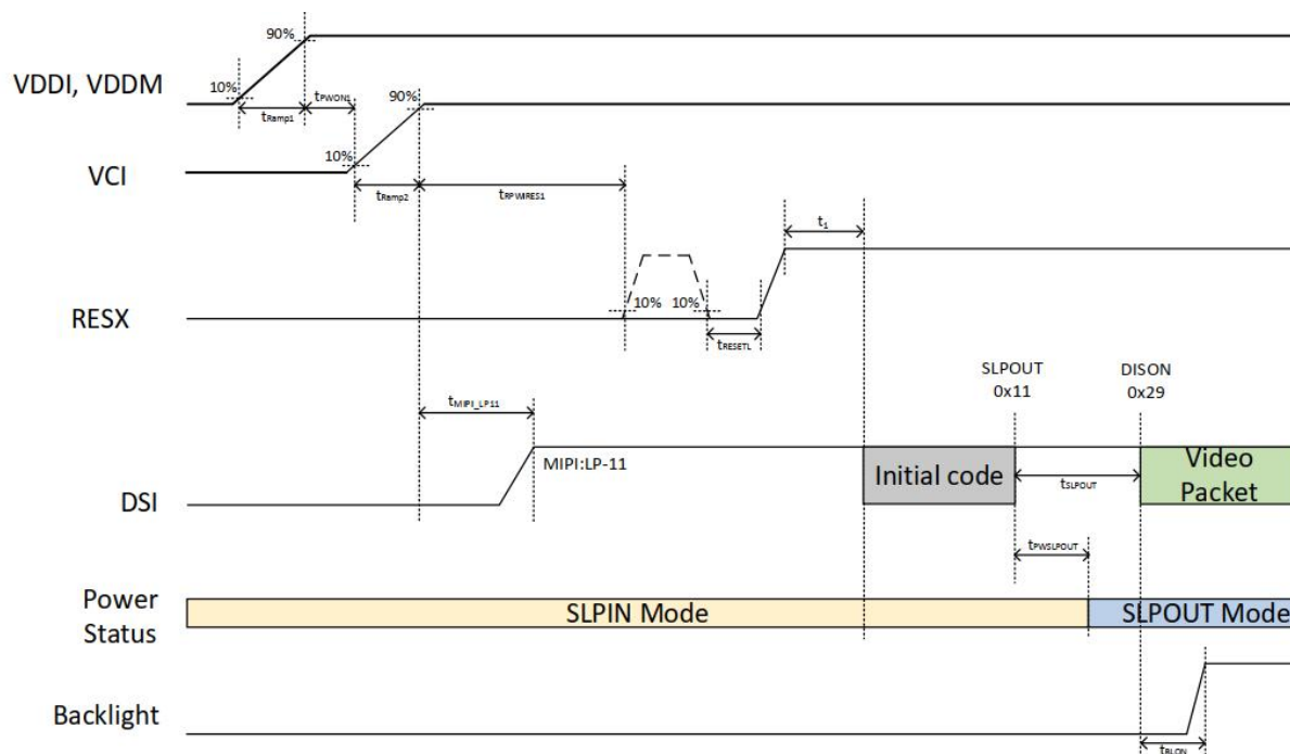
MIPI 接口上电 MIPI Interface power on
